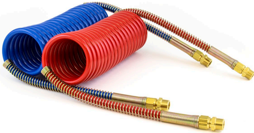
Set of 15' Coiled Air Assemblies with 40" Leads
